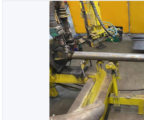
Nut welding machine – welding nuts onto steel pipes
