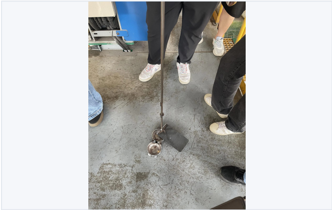
Sampling from the zinc bath with a special tool
