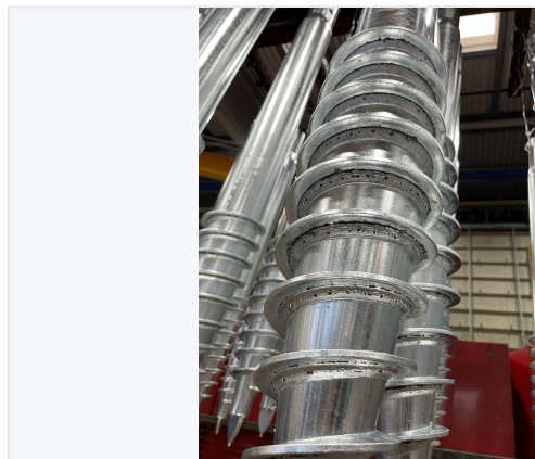
Analysis of the galvanizing quality at the weld seam
