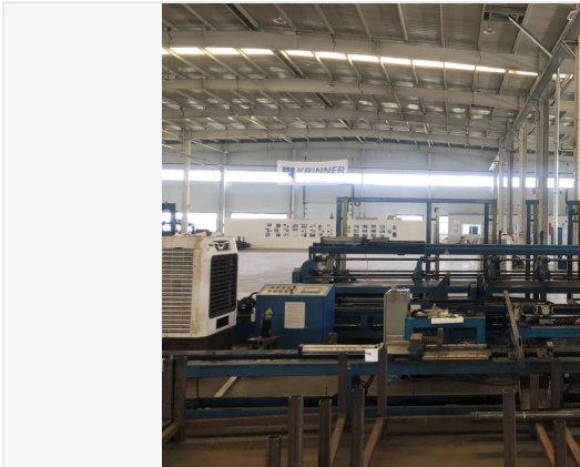
Cone machine + plasma cutting hole
